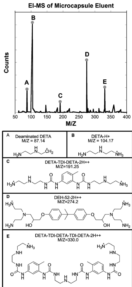
Figure 4. Electrospray mass spectrum with identified peaks.
